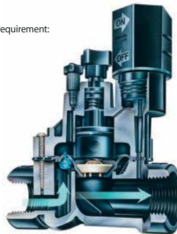
DVF Cutaway
