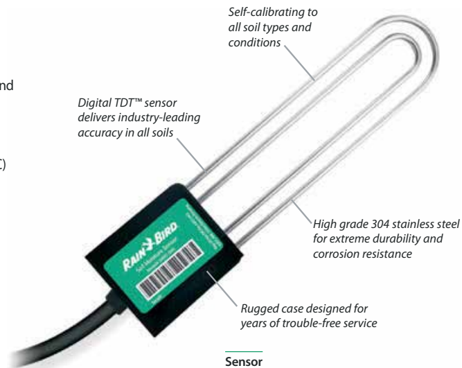
Sensor
