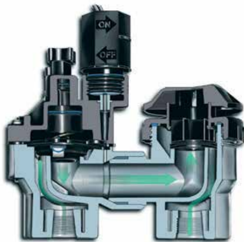
ASVF Cutaway
