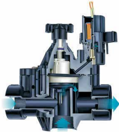
PGA Cutaway
