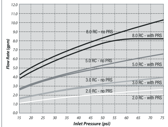
Flow Rate vs. Inlet Pressure – Rain Curtain™ Nozzles
