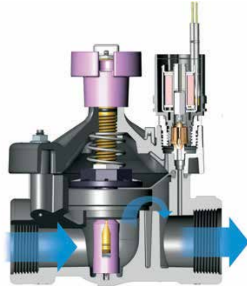
PESB-R Cutaway
