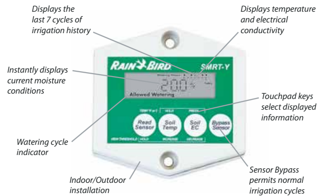
Controller Interface
