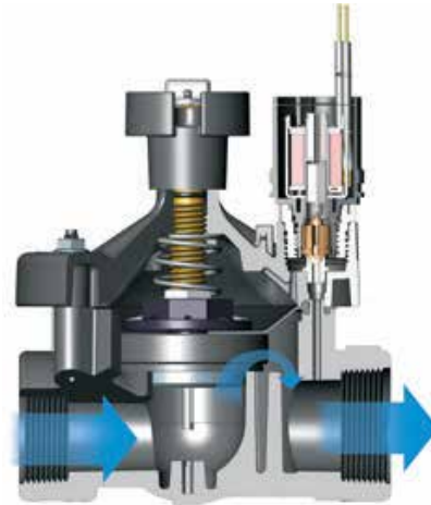
PEB Cutaway
